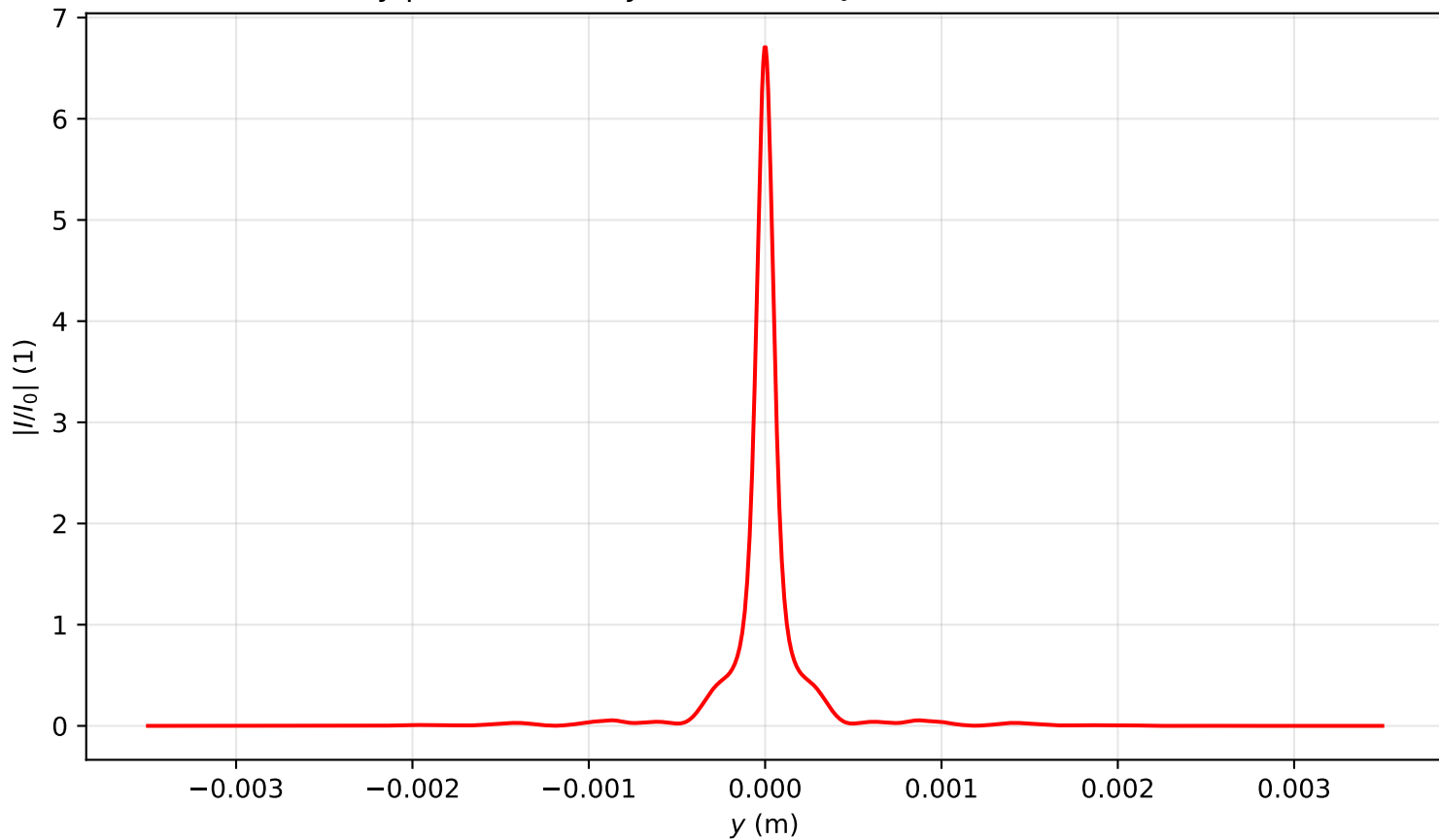
Intensity profile I(x=0, y, z=1.911)/I_0 , P_{in}=4.5P_{cr} , artificial time
